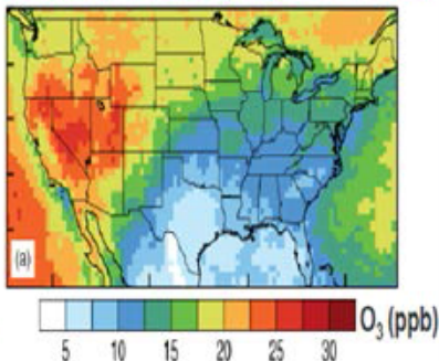
Stratospheric (O 3 S): April-June 2010
